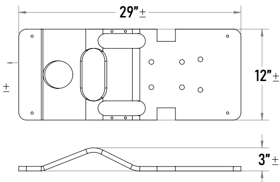
ASTM A36 15mm - 5/8" Base Total Weight: 56 lbs
