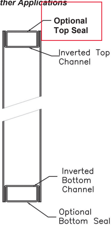
Top and Bottom Channels
